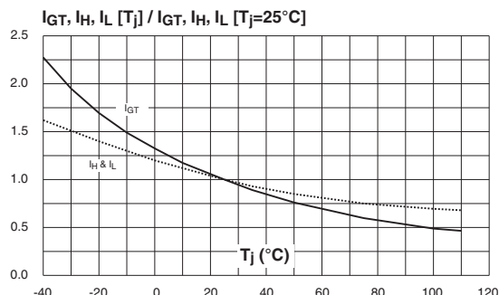
Figure 2. Relative variation of gate trigger current, holding current and latching current versus junction temperature (typical values)
