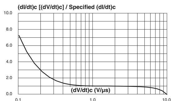
Figure 6. Relative variation of critical rate of decrease of main current versus (dV/dt)_c (typical values)
