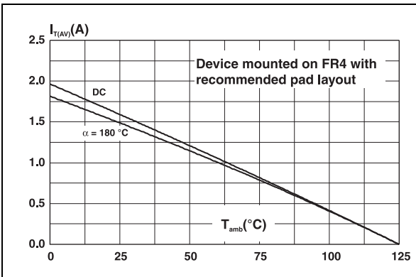
Figure 3. Average DC on-state current versus ambient temperature
